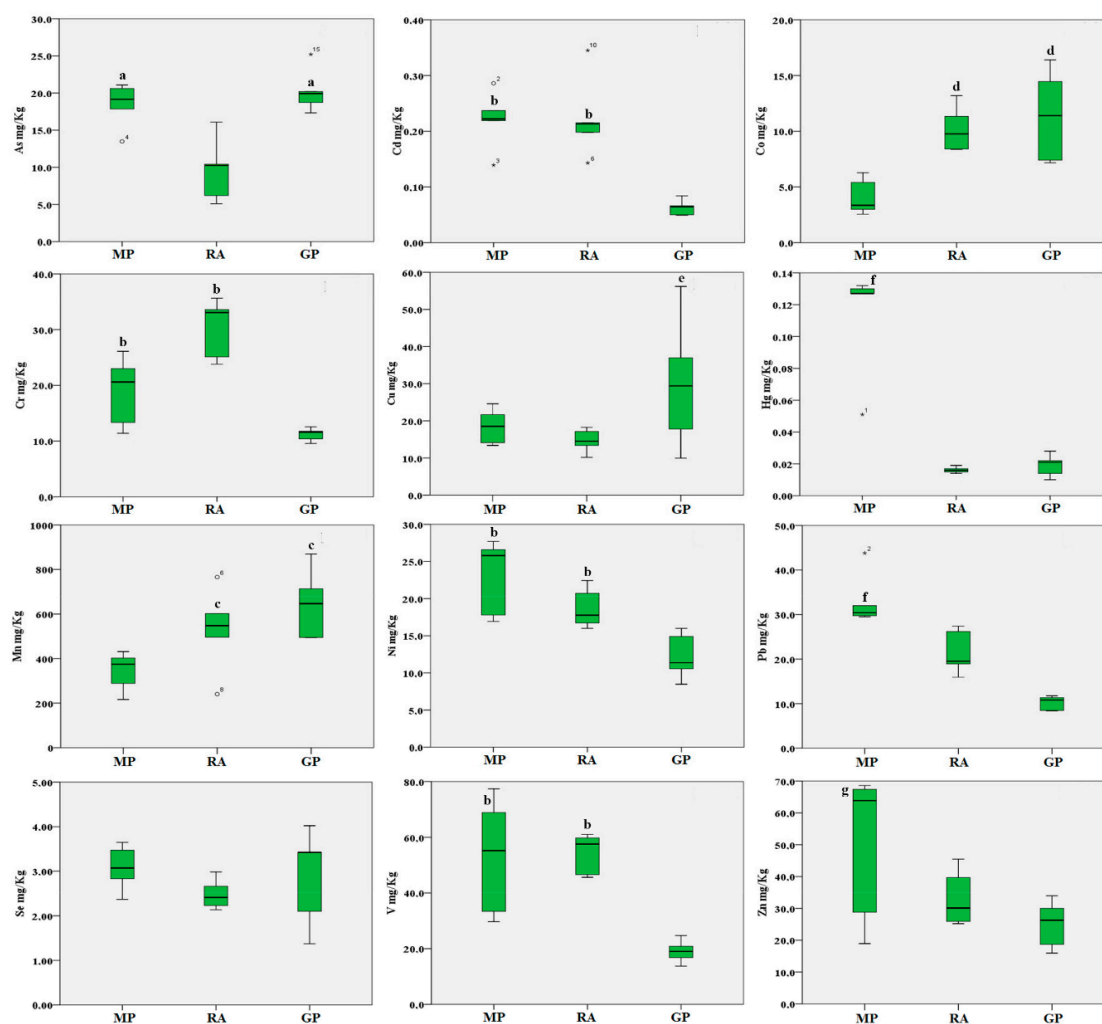
Figure 4. Boxplot of the trace elements in soil samples (mg/kg d.w.) from the three areas. MP: Magnisi peninsula; RA: Ragusa agro-ecosystem; GP: Gela plain. The box represents the interquartile (IQ) range contains the 1st quartile, the median and the 3rd quartile; whiskers represent extreme values of minimum and maximum; in addition, outliers with values between 1.5 and 3 times the IQ range are displayed. Legend: a = p < 0.05 vs. MP and GP; b = p < 0.01 vs. GP; c = p < 0.05 vs. MP; d = p < 0.01 vs. MP; e = p < 0.05 vs. MP and RA; f = p < 0.01 vs. RA and GP; g = p < 0.05 vs. RA and GP.
