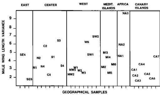
Fig. 5. Variance in male wing length for geographic samples with >20 specimens. Eurasian specimens are grouped from left to right into Eastern, Central, Western Europe and Mediterranean Islands respectively (see legend p. 821). North African samples are grouped into western Maghreb and Canary islands.
